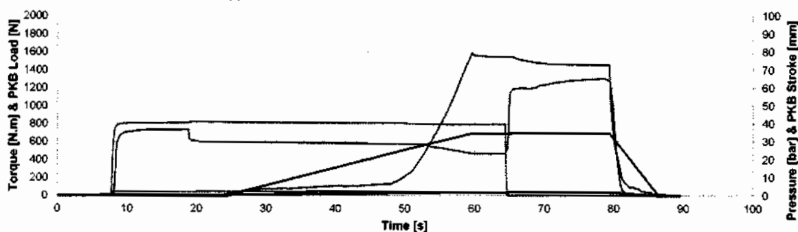
Typical curve - PKB Load 1500 N - Forward direction
