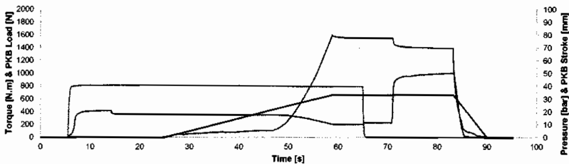
Typical curve - PKB Load 1500 N - Backward direction
